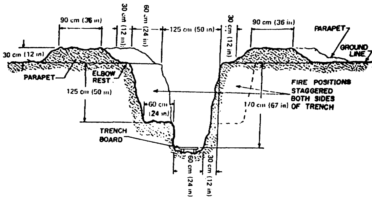
Figure 2-3. Standard trench with fighting step.
